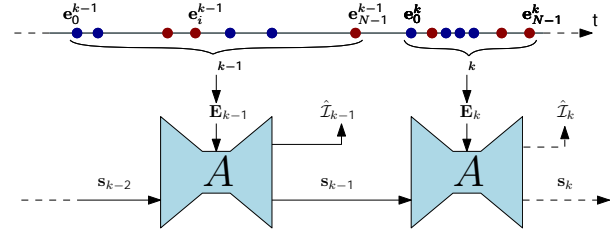
Fig. 3. Overview of our approach. The event stream (depicted as red/blue dots on the time axis) is split into windows \varepsilon_k containing multiple events. Each window is converted into a 3D event tensor \mathbf{E}_k and passed through the network, together with the previous state \mathbf{s}_{k-1} to generate a new image reconstruction \hat{\mathcal{I}}_k and updated state \mathbf{s}_k . In this example, each window \varepsilon_k contains a fixed number of events N = 7 .
